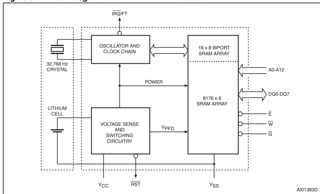
Figure 5. Block diagram of a TIMEKEEPER® device
