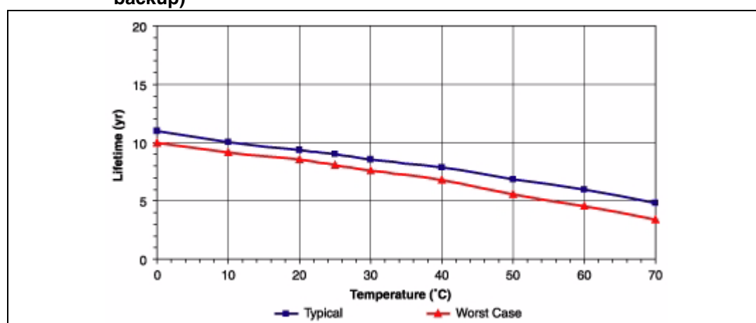
Figure 8. M48T58 data retention lifetime vs. temperature (48 mAh, 100% battery backup)
